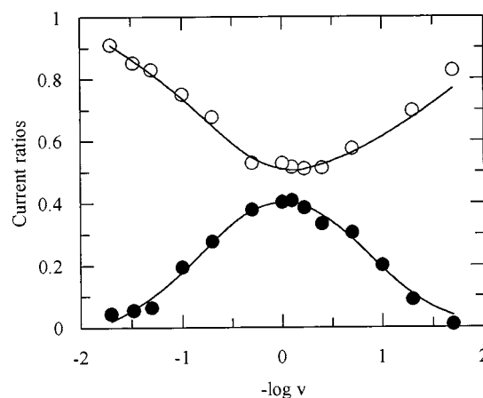
Fig. 4 Experimental (symbols) and theoretical (lines) variations of the reversibility of wave (I), i_p(cis^{+0})/i_p(cis^{0+}) , (top) and of the parameter \rho = i_p(trans^{+0})/i_p(cis^{0+}) (bottom) as a function of scan rate. The solid lines correspond to the working curves for the mechanism described in Scheme 1 where k_1 = 5 , k_{-1} = 2.5 , k_{-2} = 1 and k_2 = 0 s -1
