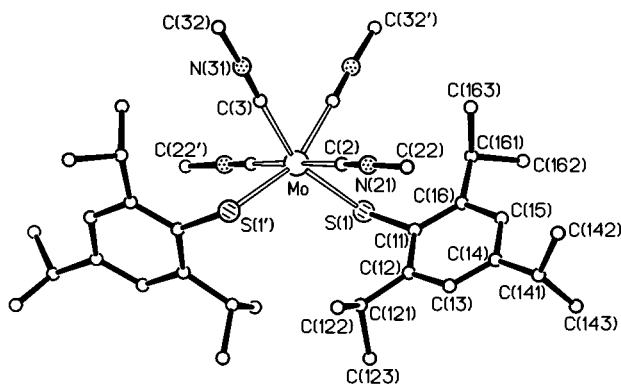
Fig. 1 View of a molecule of \text{cis-}[\text{Mo}(\text{tipt})_2(\text{CNMe})_4] 1a , showing the atomic numbering scheme. The crystal of the tungsten analogue, complex 1c , is of the opposite enantiomer, having a structure virtually identical to the mirror image of that shown here. The two-fold symmetry axis is vertical in the plane of the paper
