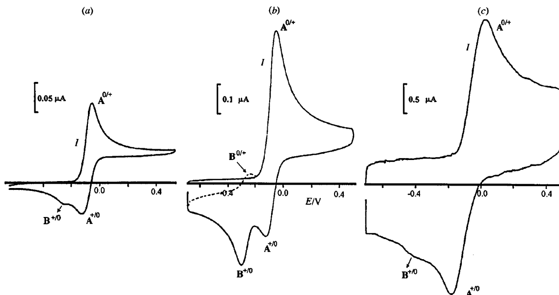
Fig. 3 Cyclic voltammograms of cis -[Mo(tipt) 2 (CNBu) 4 ] (1.13 mM, in CH 2 Cl 2 with 0.2 M [NBu 4 ][BF 4 ]) at -50 °C and at a platinum-disc ( d = 0.5 mm) working electrode. Potentials are given in V vs. SCE; A and B denote the cis and trans isomers, respectively (see text). Scan rate: 0.05 (a), 0.8 (b) and 20 V s -1 (c)
